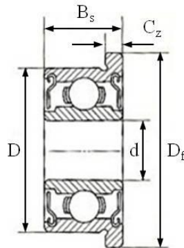
Flanged Bearing
